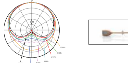
Polar Pattern d:fine™ Directional
